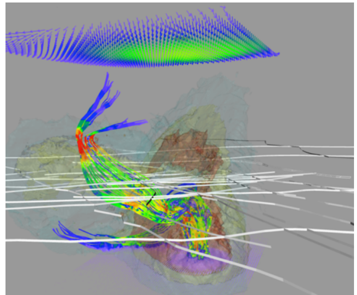
Very significant damage, as well as a high flow system evolves at the confluence of major fault structures due to fluid influx through the magma chamber at the bottom of the image.
