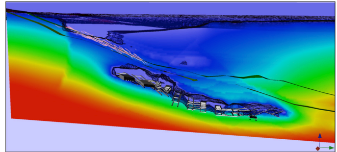
Hydraulic interconnectivity as a result of excavation-induced damage and drawdown
