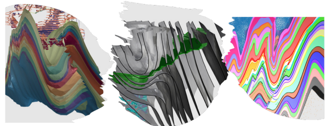
Hydrogeological and geotechnical anisotropy are realistically represented to provide an accurate overview of the hydraulic interconnections.
